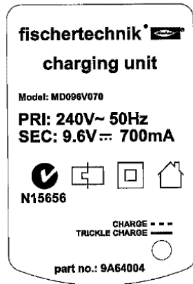
Typenschild/ ratingplate M/ scale 2:1
