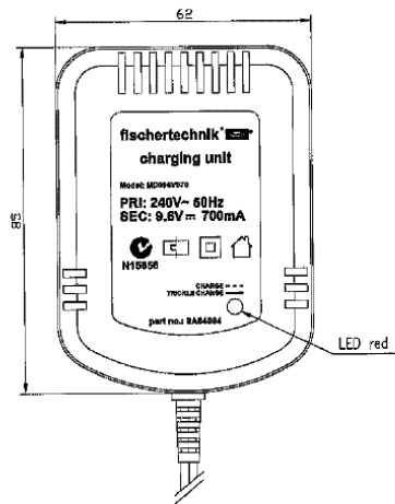
Typenschild/ ratingplate M/ scale 2:1
